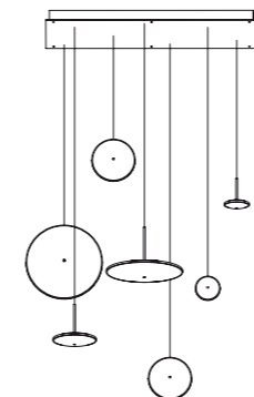
Chrona 7 Single rectangular canopy 7 pendants 2m drop
