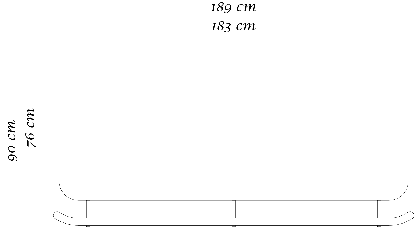
TOP VIEW
