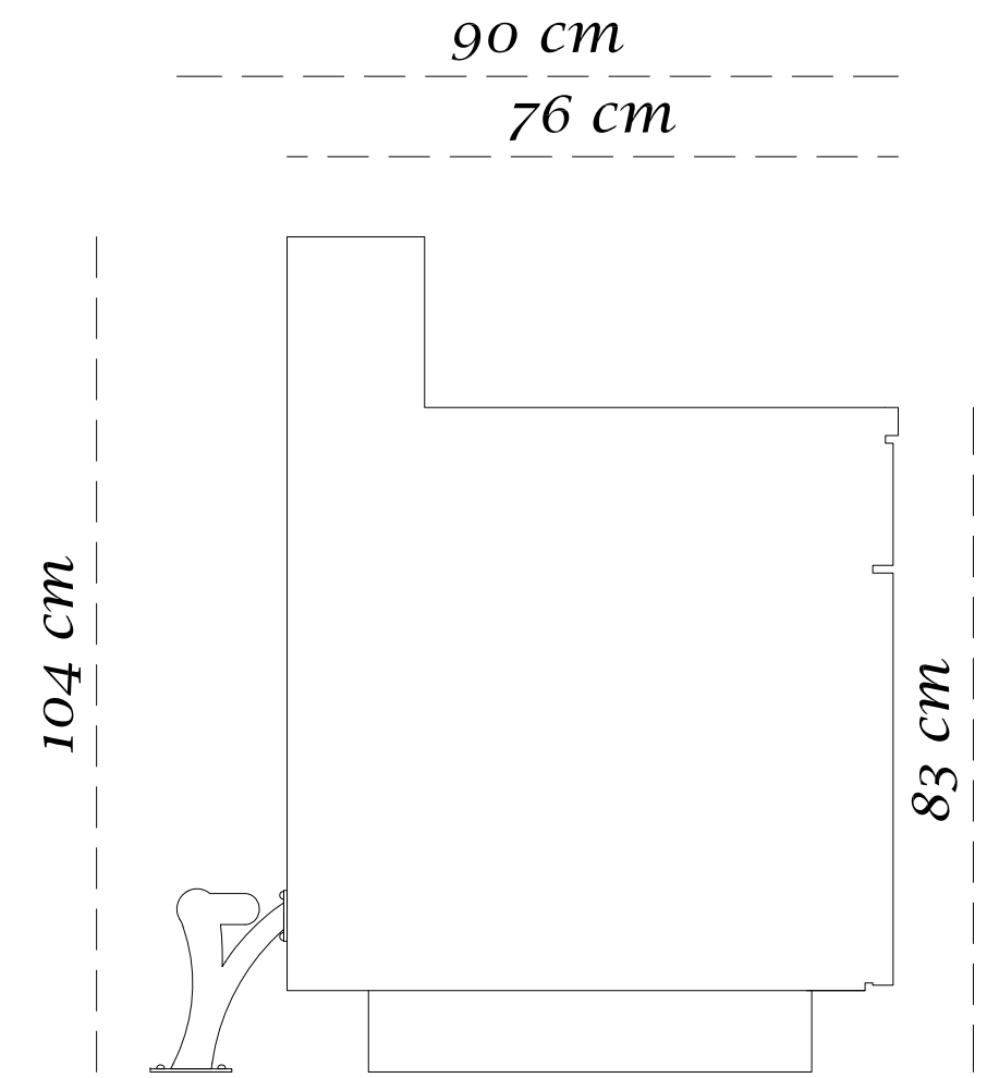
SIDE VIEW
