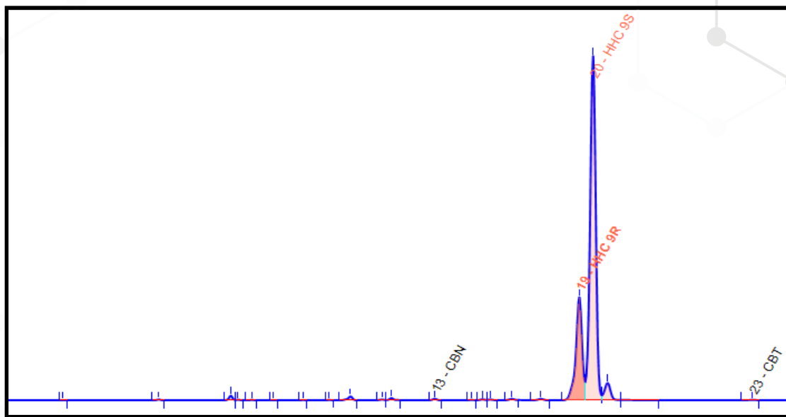
Figure 1. UHPLC-PDA chromatogram of The Dopest Peach HHC Gummies
