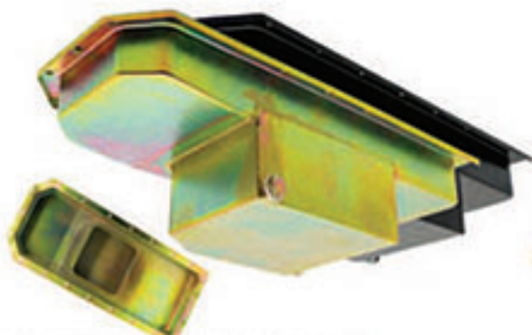
HEMI SWAP MID SUMP OIL PAN - GEN 3 2003-19 Gen 3 Hemi 5.7L, 6.1L, 6.4L Engine Swaps for 1963-75 Mopar A, B, C & E Body cars. 7qt Capacity. HZ-7479-Z Zinc HZ-7479-PBK Black
