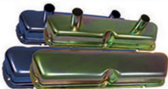
FORD VALVE COVERS - CIRCLE TRACK 1962-85, 260-289-302-351W BAFFLED HZ-7225-Z Zinc HZ-7225-PBL Blue TALL H: 3-1/2"
