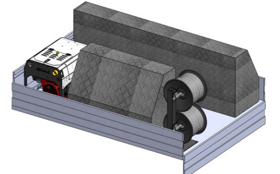
4.1 Ute - Setup 1
