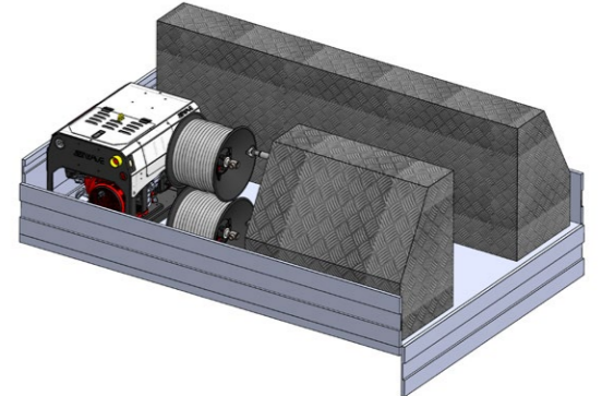
4.2 Ute - Setup 2
