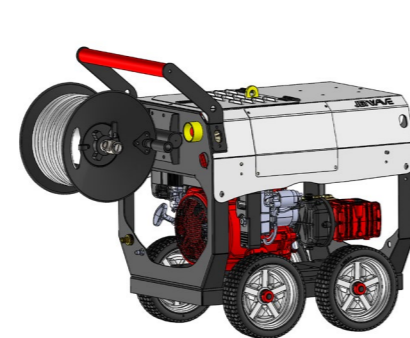
2.1 Trolley - Front Hose Reel
