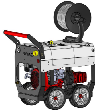
2.2 Trolley - Top Hose Reel
