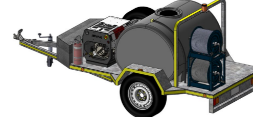
3.1 Trailers - Single Axle 1000L (Hornet G2D Shown with Mine Spec Upgrade)
