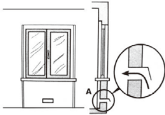
Examples of ventilation holes for comburent air.
