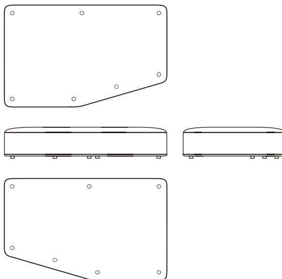
12002-46-2 Causeway module 6 RHF W2200 D1050/1380 H420
