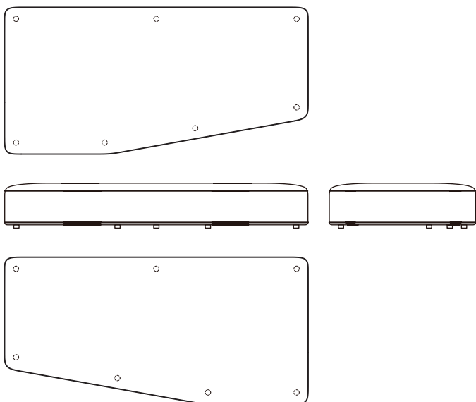
12002-44-2 Causeway module 4 RHF W2850 D1050/1380 H420
