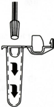
Fig. 1 Insert wires to bottom of gel-filled tube.
