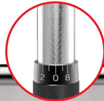
HEAVY-DUTY WRENCH FEATURES A 10 TO 150 FOOT POUND RANGE.
