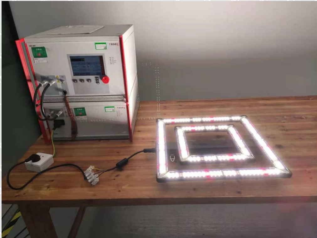
7.9 Photograph – Injected Currents Immunity Test Setup
