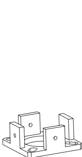
Concealed base for invisible mounting on concrete base or paved surface
