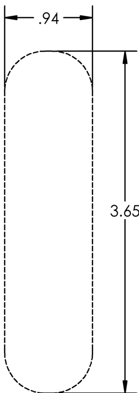
MOUNT FOOTPRINT
