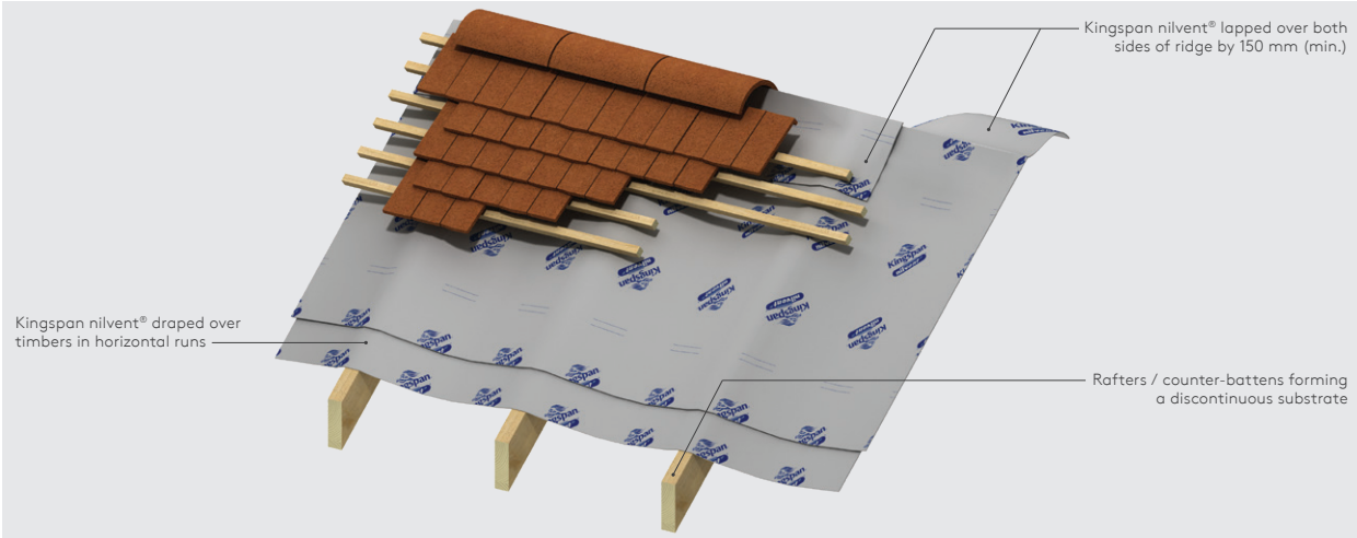
Figure 7b - Ridge - draped horizontal installation
