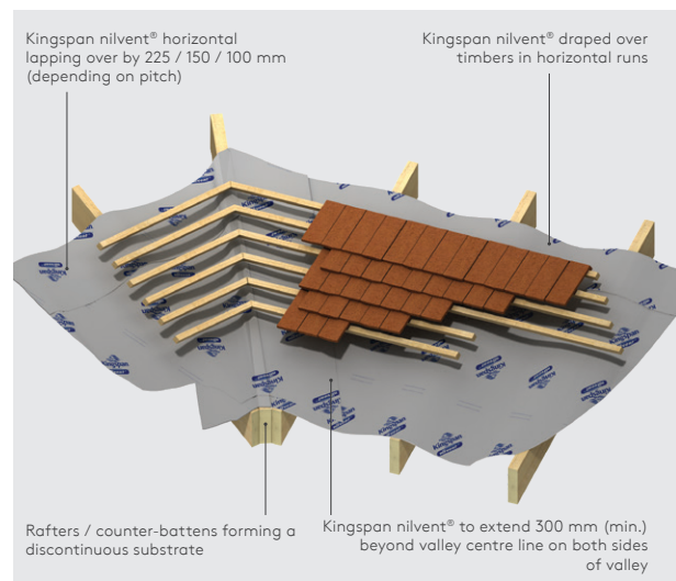
Figure 11d - Valleys - draped horizontal installation
