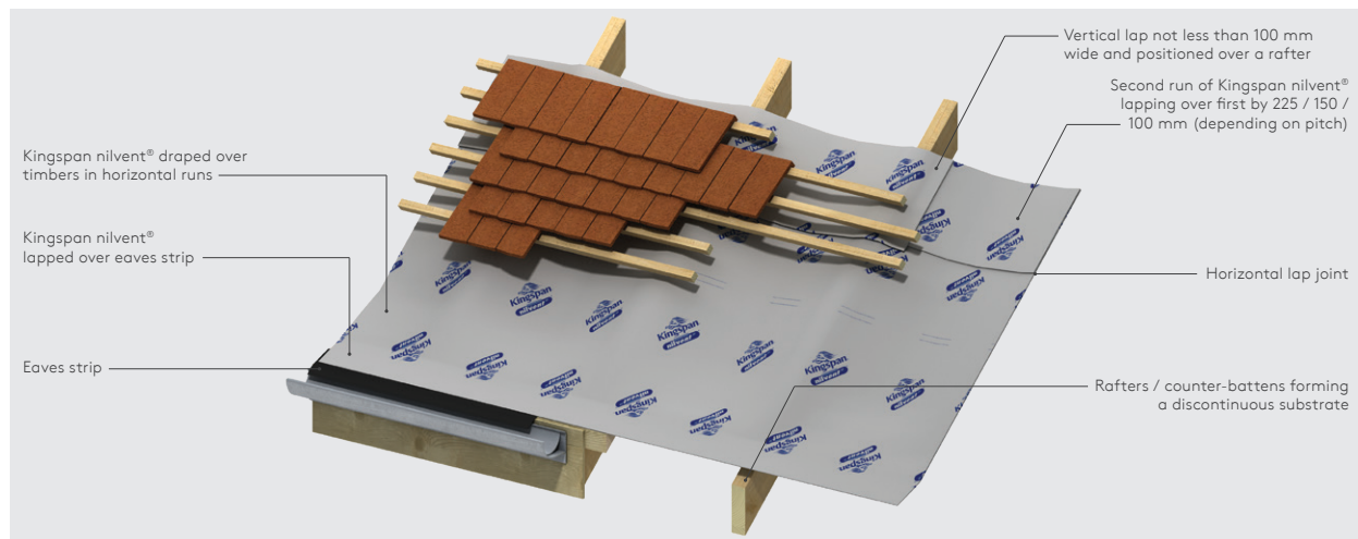
Figure 7a - Eaves - draped horizontal installation
