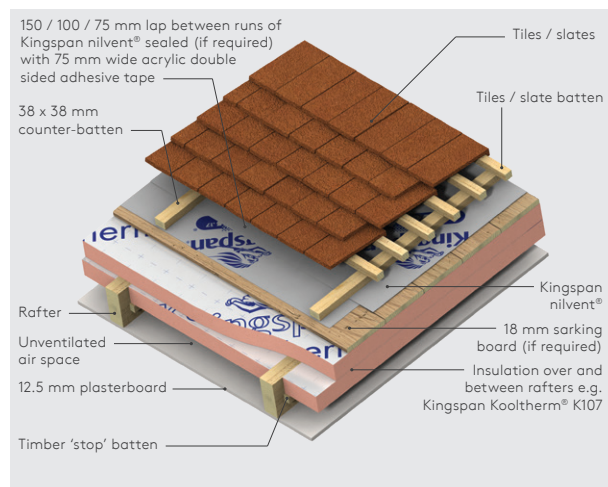
Figure 1b - Insulation over rafters - sarking board / no sarking board - battens & tiles
