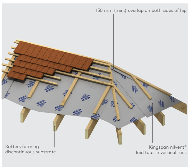
Figure 10c - Hips - vertical installation
