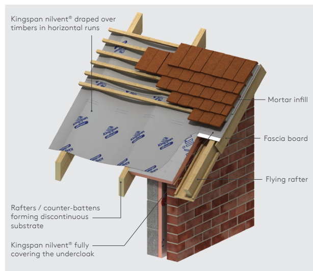
Figure 9d - Verges - draped horizontal installation
