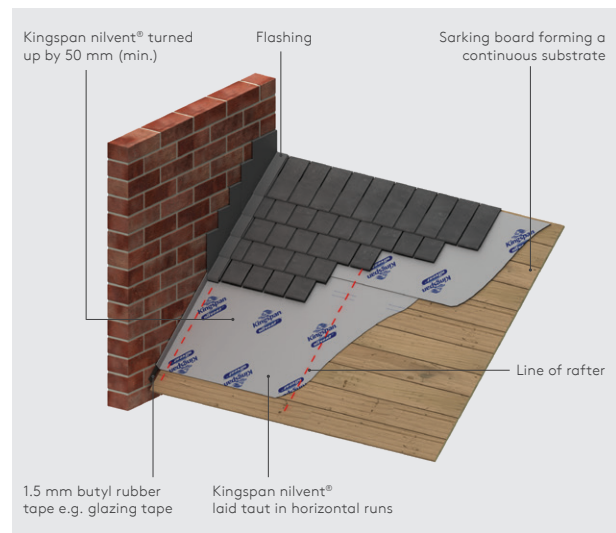
Figure 8b - Abutments - fully supported horizontal installation with natural slates
