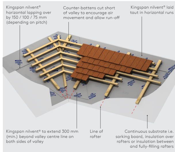
Figure 11a - Valleys - fully supported horizontal installation
