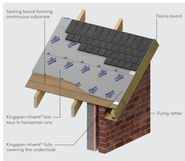
Figure 9b - Verges - fully supported horizontal installation with natural slates
