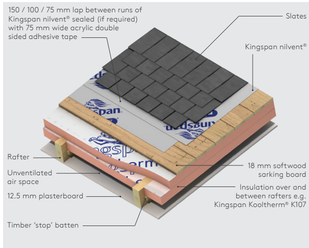
Figure 1e - Insulation over rafters - sarking board and natural slates
