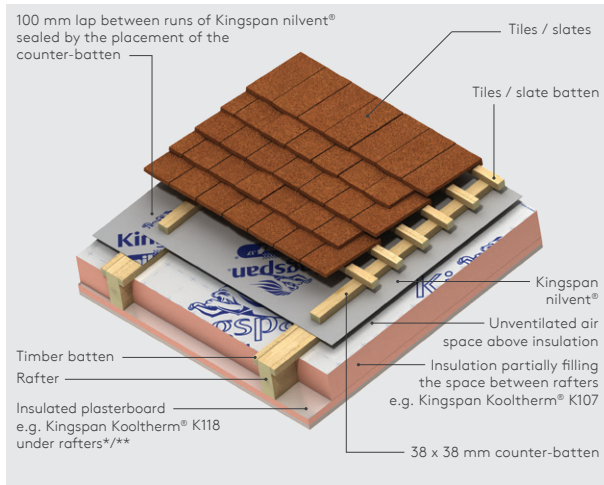
Figure 2 - Partially filled insulation between rafters - no sarking board - battens & tiles
