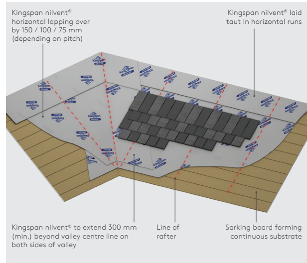
Figure 11b - Valleys - fully supported horizontal installation with natural slates
