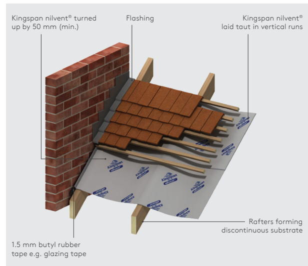
Figure 8d - Abutments - draped horizontal installation
