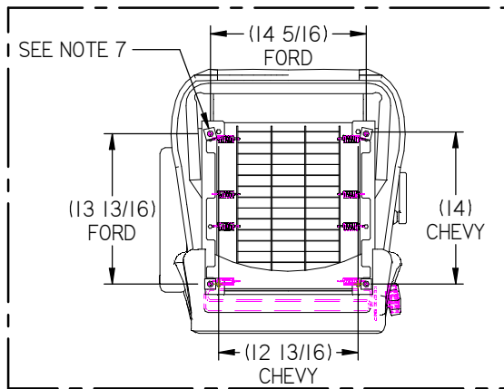
VIEW B-B
