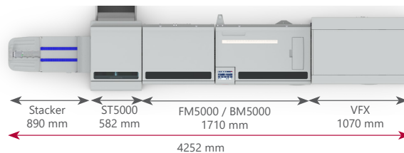
BM5000 System with ST5000 - Machine footprint
