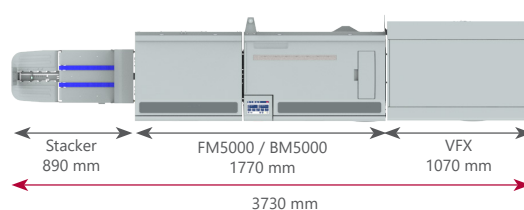
BM5000 System with VFX feeder - Machine footprint
