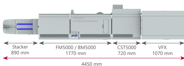
BM5000 System with CST5000 - Machine footprint
