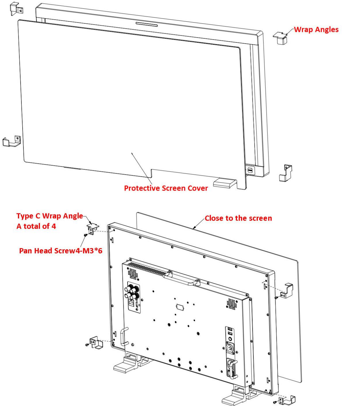
Figure 5.2-12 Mount a Protective Screen for LCM230-E
