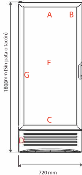
Vista frontal
