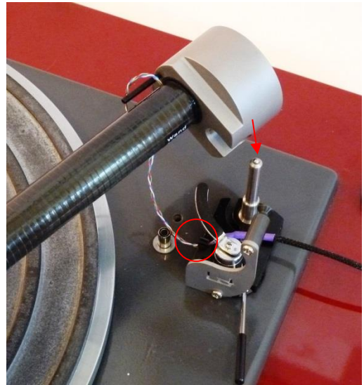
5. Feed wire thru clip and place arm
