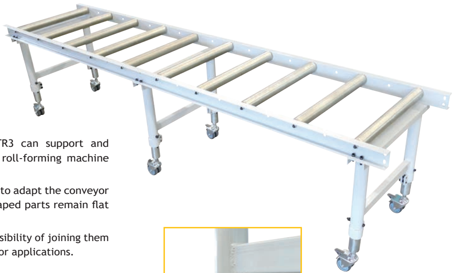
Model Ref. TR3 with optional swivel casters Ref. TR3-ROUL
