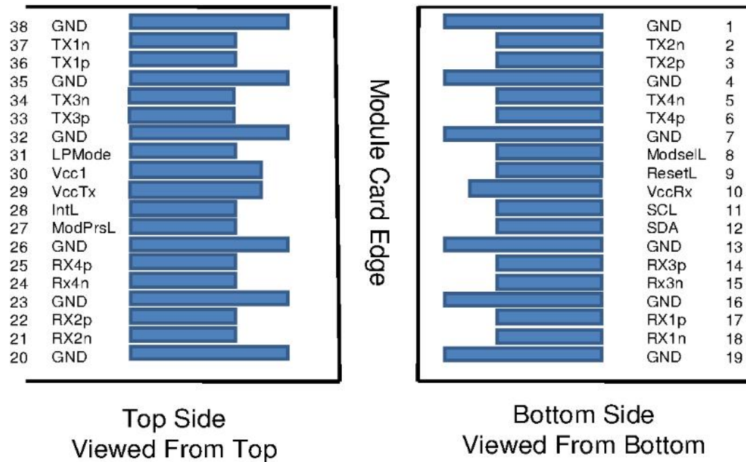
Figure 1.Electrical Pin-out Details
