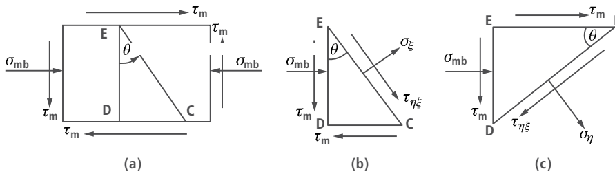
Fig. 9.16 Determination of stresses on planes parallel and perpendicular to the plane of the buckle.
