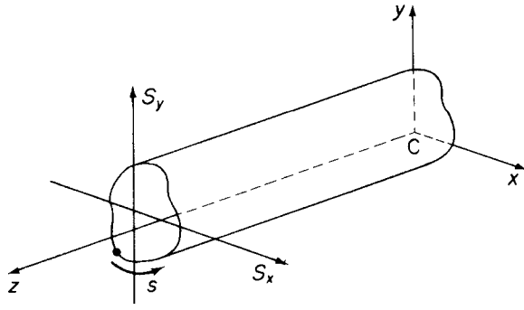
Fig. 17.10 Shear of closed section beams.
