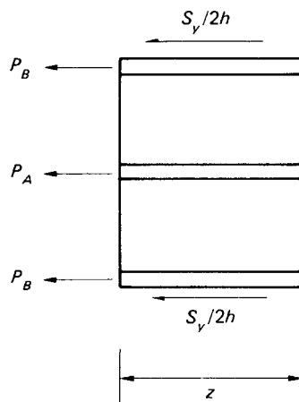
Fig. 26.15 Equilibrium of element of central boom.
