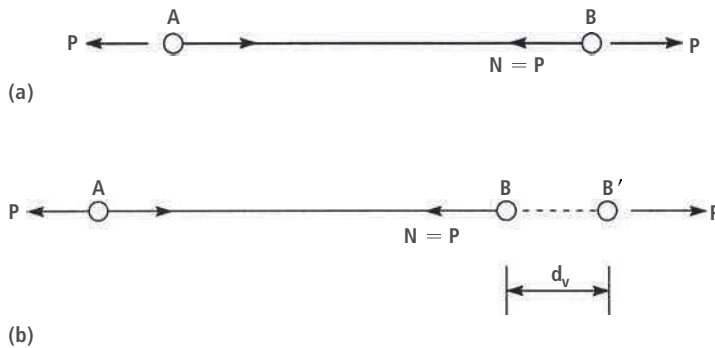
Fig. 4.6 Sign of the internal virtual work in an axially loaded member.
