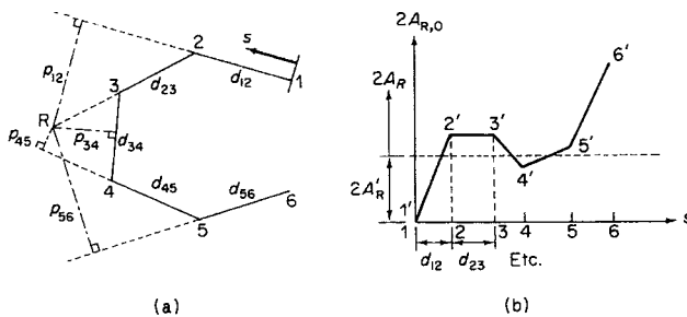
Fig. 27.8 Computation of torsion bending constant \Gamma_R : (a) dimensions of flat-sided open section beam (b) variation of 2A_{R,0} around beam section.
