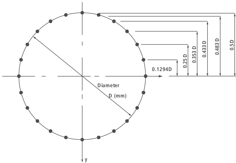
Fig. A.8 Idealized fuselage cross-section.
