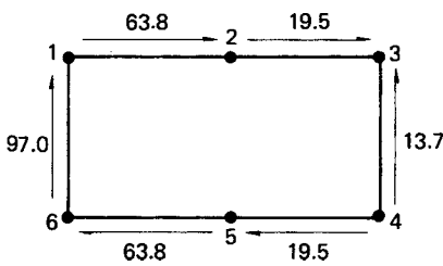
Fig. 21.8 Shear flow (N/mm) distribution in beam section of Example 21.2.
