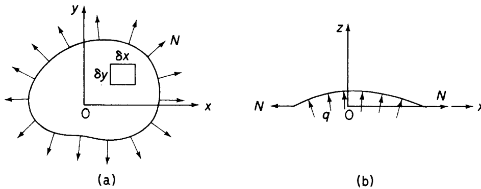
Fig. 3.7 Membrane analogy: in-plane and transverse loading.
