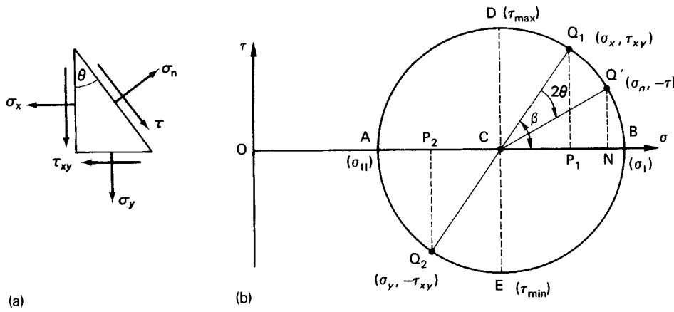
Fig. 1.12 (a) Stresses on a triangular element (b) Mohr's circle of stress for stress system shown in (a).
