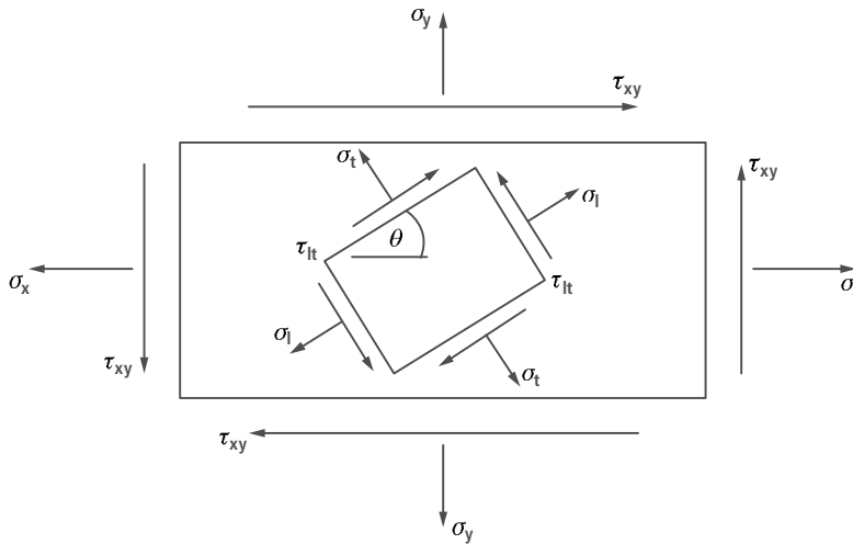
Fig. 25.8 Stresses in a generally orthotropic ply.
