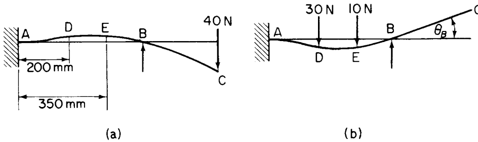
Fig. 5.27 (a) Given deflected shape of propped cantilever; (b) determination of the deflection of C.
