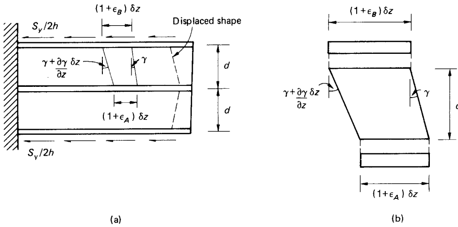
Fig. 26.17 Compatibility condition.
