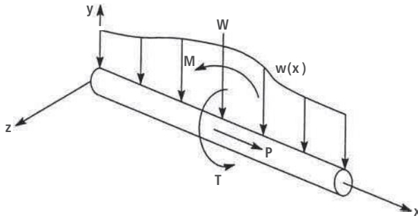
Fig. 4.7 Virtual work due to externally applied loads.
