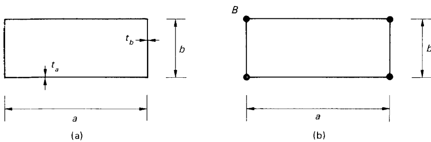
Fig. 26.5 Idealization of a rectangular section beam subjected to torsion: (a) actual (b) idealized.
