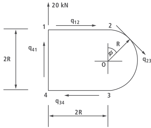
Fig. 26.4 Beam section of Example 26.2.
