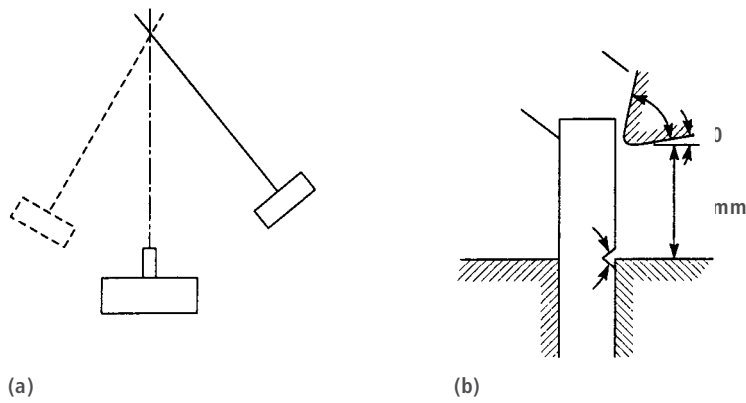
Fig. 11.7 Izod impact test.
