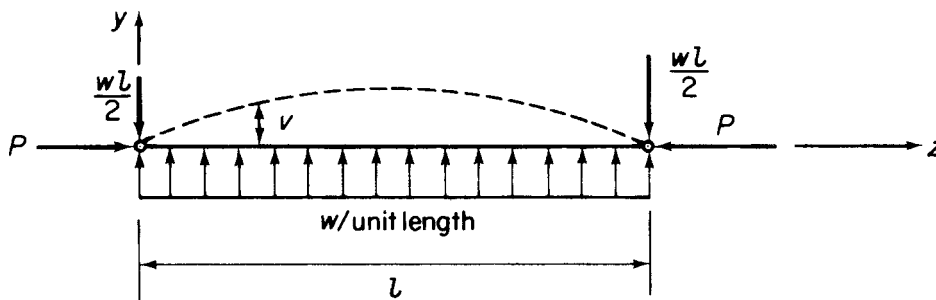
Fig. 8.11 Bending of a uniformly loaded beam-column.
