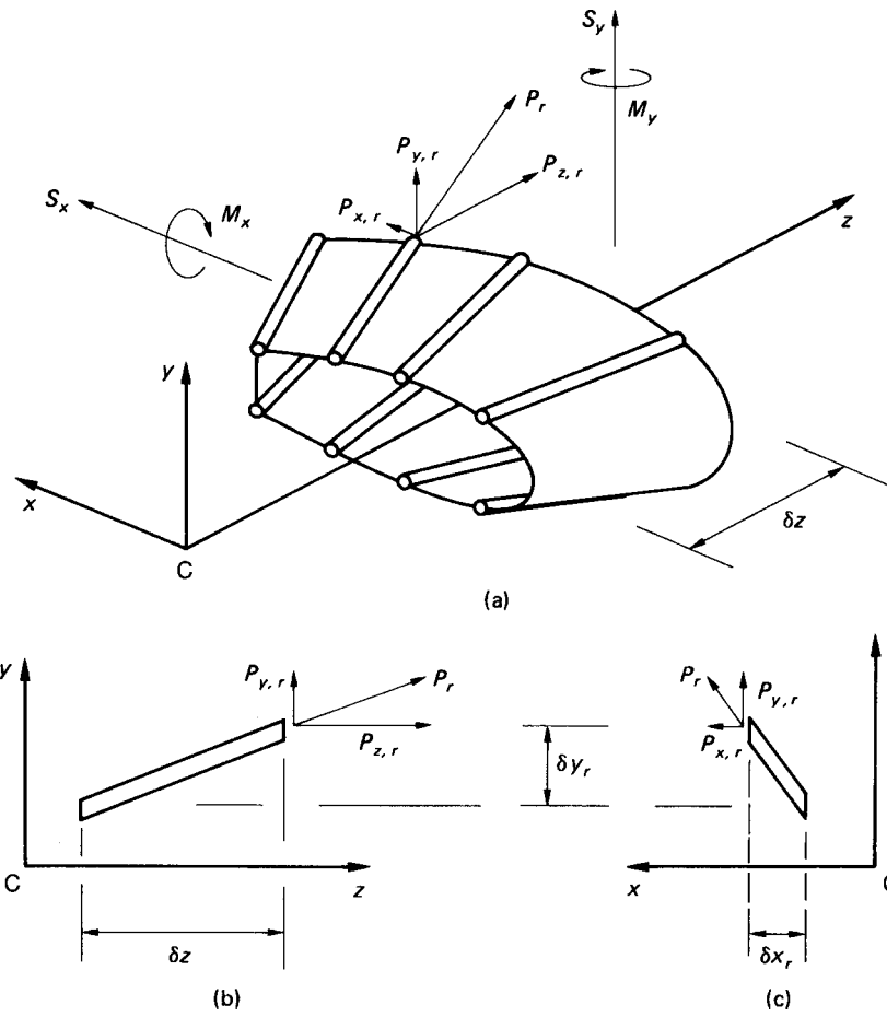
Fig. 21.4 Effect of taper on the analysis of open and closed section beams.
