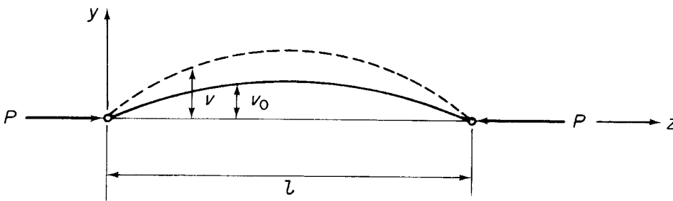
Fig. 8.9 Initially bent column.
