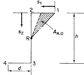
Fig. 27.15 Calculation of axial constraint shear flows.
