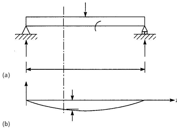
Fig. 16.19 Deflection of a simply supported beam carrying a concentrated load at mid-span (Example 16.8).
