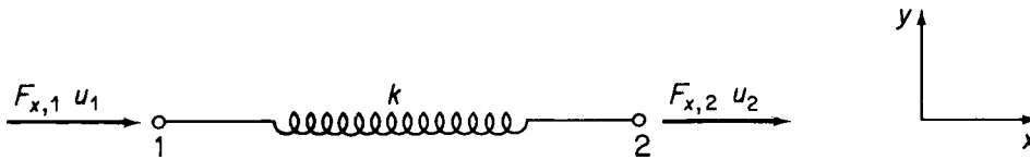
Fig. 6.1 Determination of stiffness matrix for a single spring.
