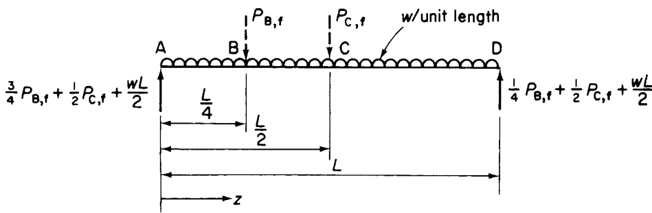
Fig. 5.7 Deflection of a simply supported beam by the method of complementary energy.
