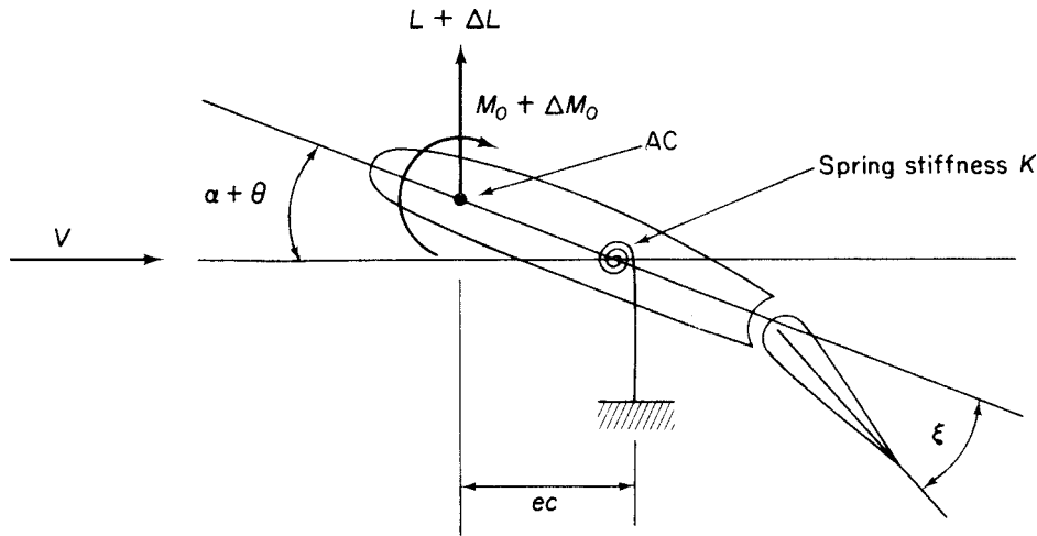
Fig. 28.5 Aileron effectiveness and reversal speed (two-dimensional case).
