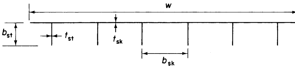
Fig. 9.5 Stiffened panel.
