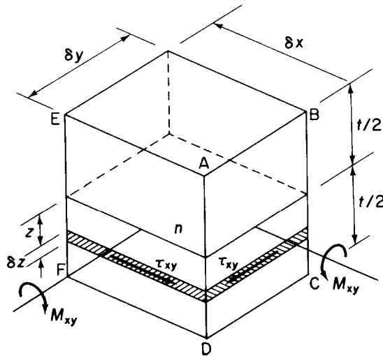
Fig. 7.6 Complementary shear stresses due to twisting moments M_{xy} .
