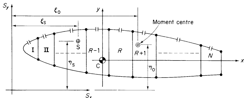
Fig. 23.8 N-cell wing section subjected to shear loads.
