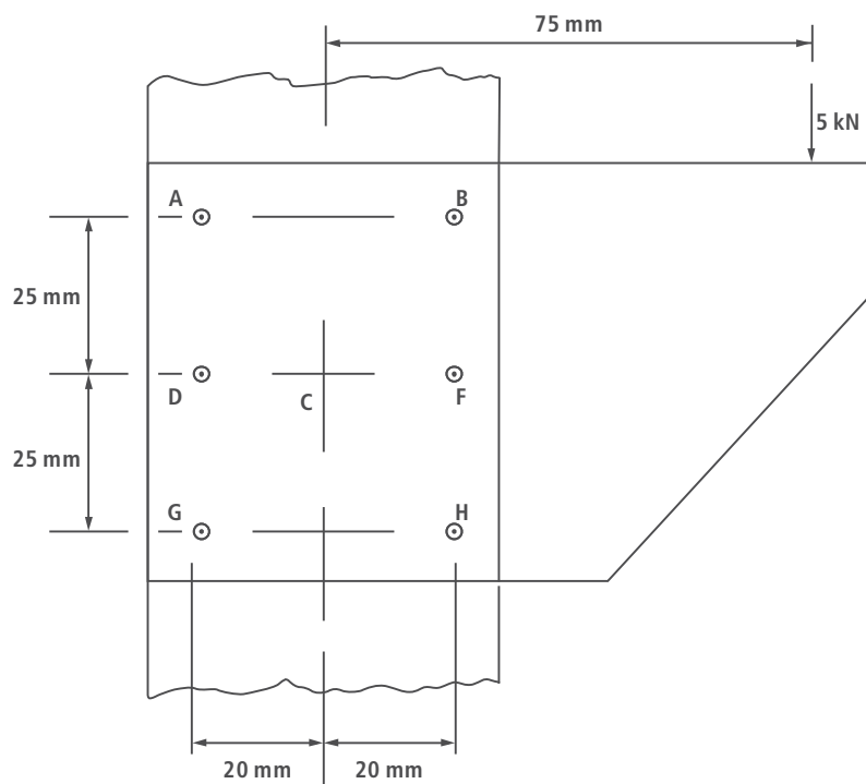
Fig. 12.15 Joint of Example 12.2.
