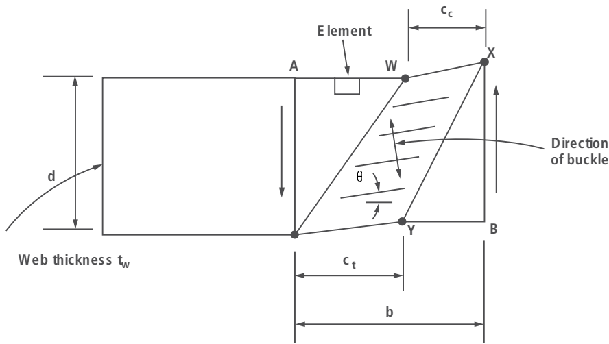
Fig. 9.15 Collapse mechanism of a panel of a tension field beam.
