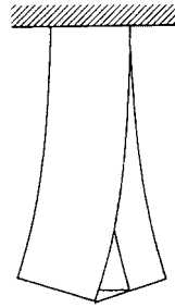
Fig. 27.3 Bending effect of axial constraint on flanges of I-section beam subjected to torsion.
