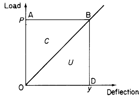
Fig. 5.2 Load-deflection curve for a linearly elastic member.
