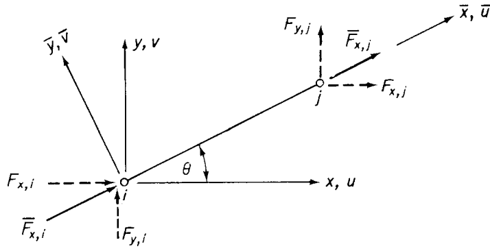
Fig. 6.3 Local and global coordinate systems for a member of a plane pin-jointed framework.
