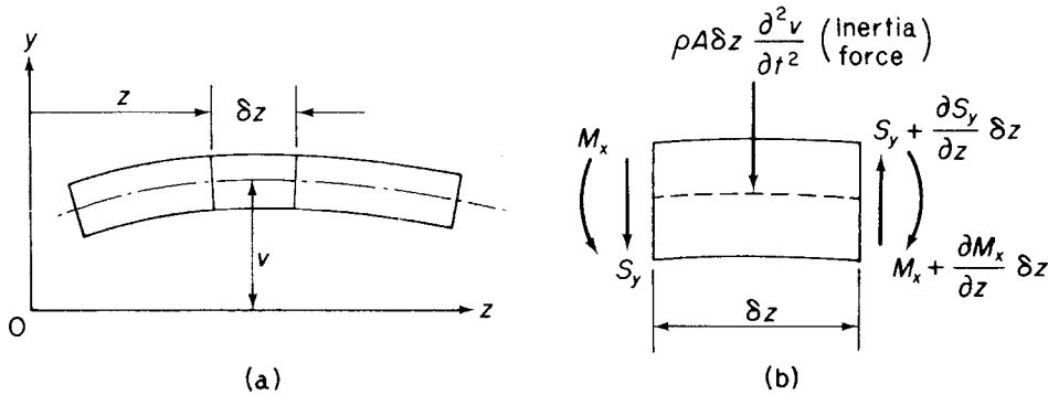
Fig. 10.9 Vibration of a beam possessing mass.
