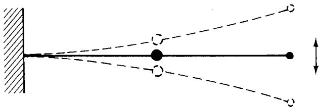
Fig. 10.4 The first natural mode of the mass/beam system of Fig. 10.3.
