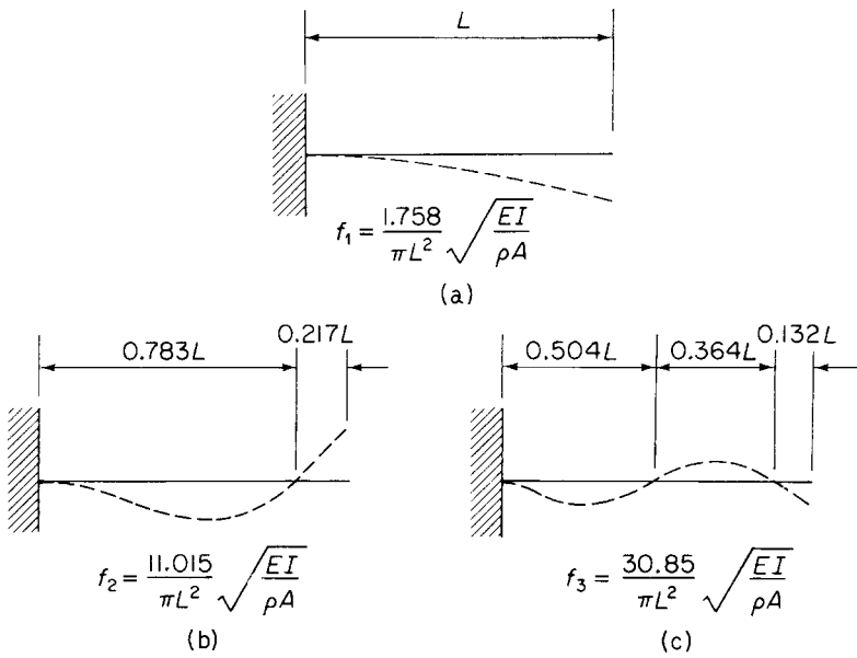
Fig. 10.13 The first three normal modes of vibration of the cantilever beam of Example 10.5.
