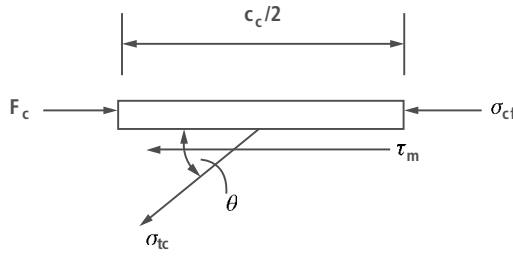
Fig. 9.18 Determination of flange stress.
