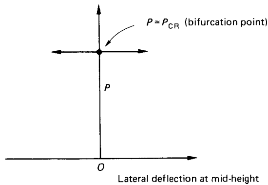
Fig. 8.4 Behaviour of a perfect pin-ended column.
