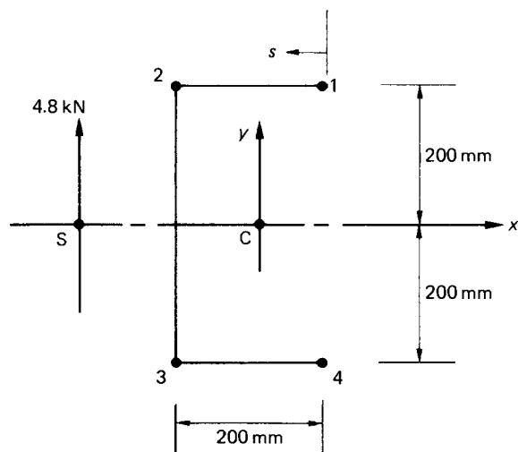
Fig. 20.7 Idealized channel section of Example 20.3.
