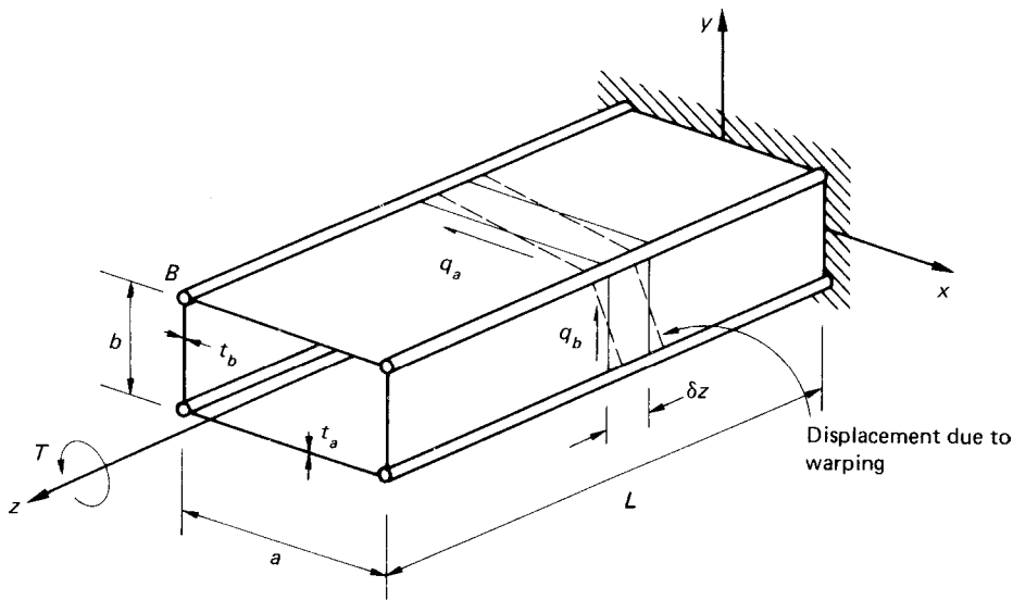
Fig. 26.6 Idealized rectangular section beam built-in at one end and subjected to a torque at the other.
