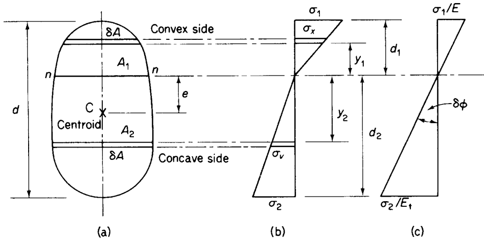
Fig. 8.8 Determination of reduced elastic modulus.
