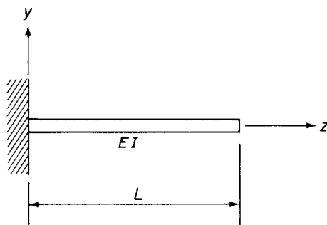
Fig. 10.12 Cantilever beam of Example 10.5.
