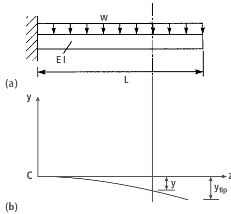
Fig. 16.17 Deflection of a cantilever beam carrying a uniformly distributed load.
