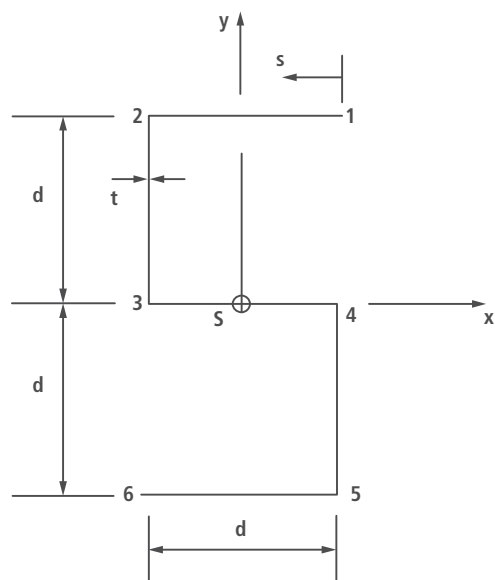
Fig. 8.19 Section of column of Example 8.5.
