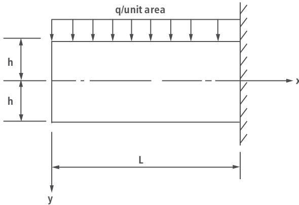
Fig. 2.3 Beam of Example 2.3.
