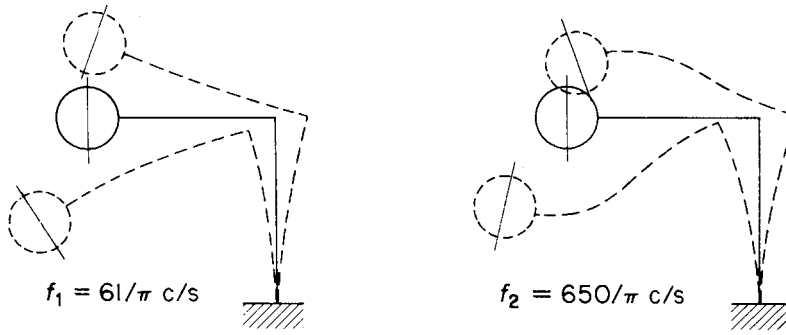
Fig. 10.8 The first two natural modes of vibration of the beam/mass system of Fig. 10.7.
