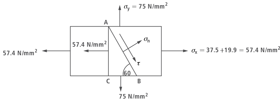
Fig. 1.9 Element of Example 1.1.
