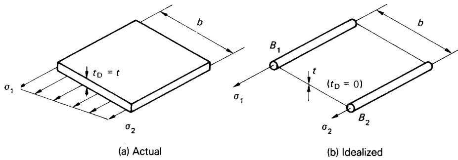
Fig. 20.3 Idealization of a panel.
