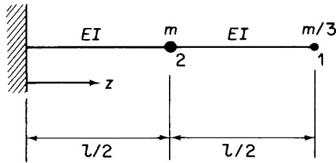
Fig. 10.3 Mass/beam system for Example 10.1.
