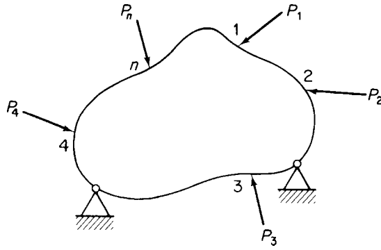
Fig. 5.26 Linearly elastic body subjected to loads P_1, P_2, P_3, \dots, P_n .
