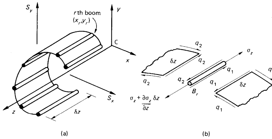
Fig. 20.6 (a) Elemental length of shear loaded open section beam with booms (b) equilibrium of boom element.
