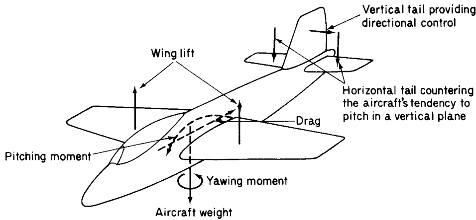
Fig. 12.1 Principal aerodynamic forces on an aircraft during flight.
