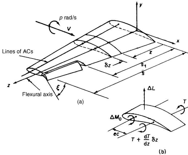
Fig. 28.6 Aileron effectiveness and reversal speed (finite wing).
