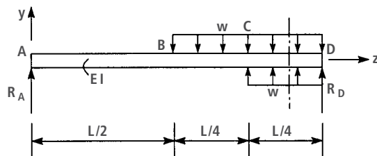
Fig. 16.22 Method of solution for a part span uniformly distributed load.
