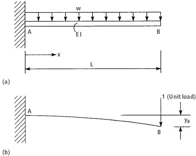
Fig. 4.10 Deflection of the free end of a cantilever beam using the unit load method.
