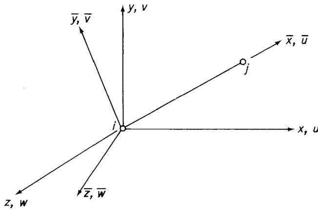
Fig. 6.5 Local and global coordinate systems for a member in a pin-jointed space frame.
