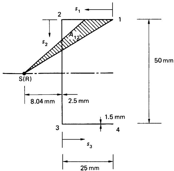
Fig. 18.14 Determination of points of zero warping.
