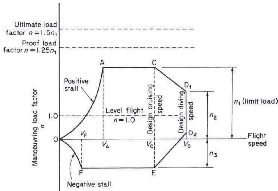
Fig. 13.1 Flight envelope
