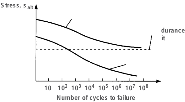
Fig. 11.21 Stress–endurance curves.
