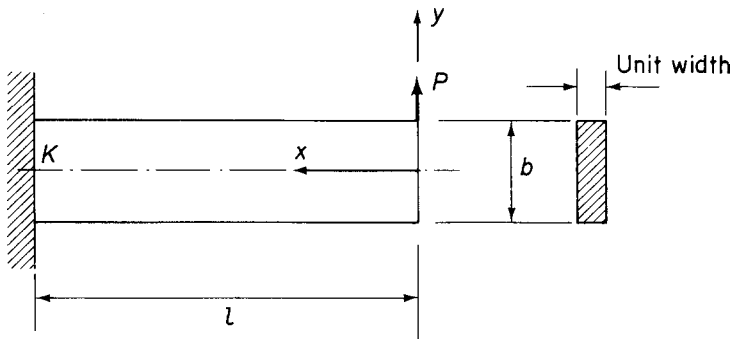
Fig. 2.6 Bending of an end-loaded cantilever.
