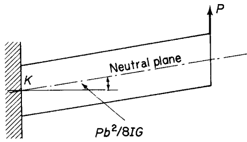
Fig. 2.7 Rotation of neutral plane due to shear in end-loaded cantilever.
