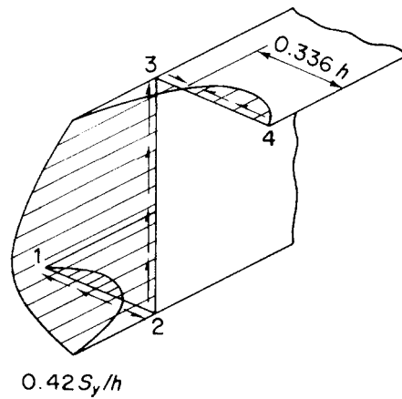
Fig. 17.7 Shear flow distribution in y -section of Example 17.1.
