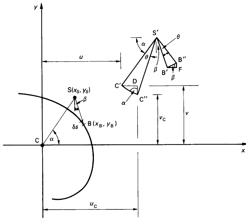
Fig. 8.16 Flexural torsional buckling of a thin-walled column.
