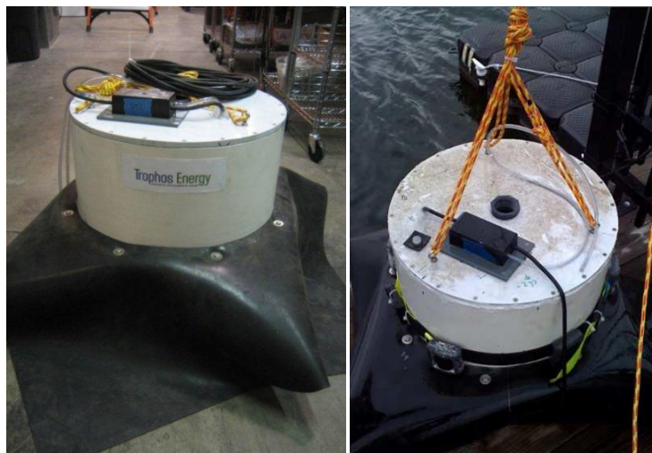
Figure 3. Photographic images of Trophos Gen. 3 BMFC in the laboratory and during field deployment.
