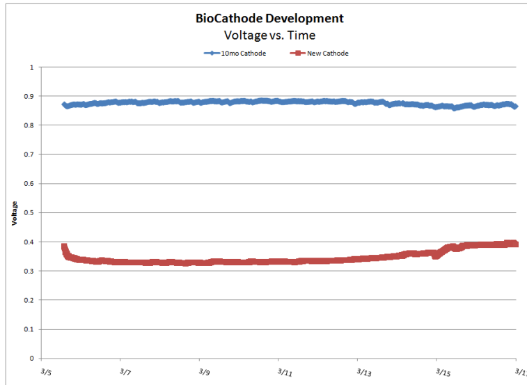
Figure 8. Performance comparison between a biocathode and a biofilm-free cathode.
