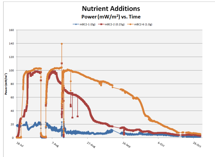
Figure 6. Effect of nutrient additions on BMFCs
