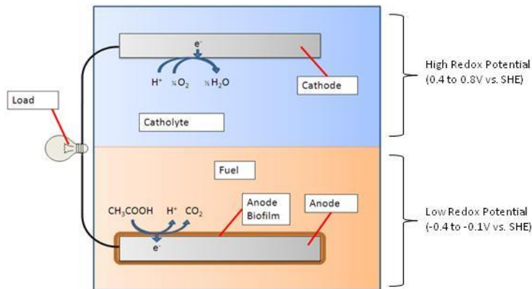
Figure 1. Graphical representation of a microbial fuel cell. Electrical energy is harvested from electrodes located in spatially separated Reduction/Oxidation reactions.
