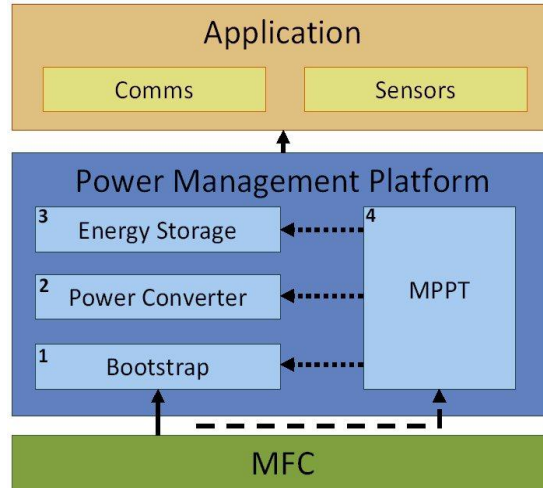
Figure 10. Block diagram of MFC power management platform
