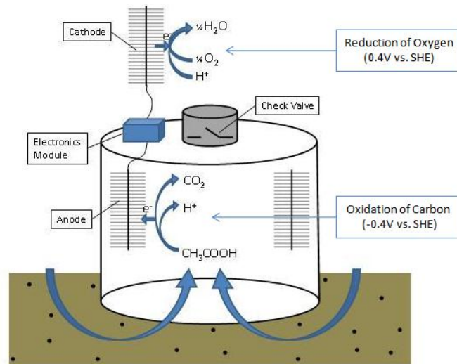
Figure 2. Benthic Chamber MFC Architecture
