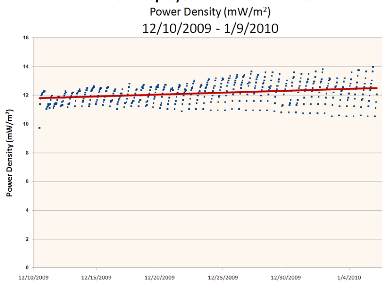
Figure 4. Data from the deployment of Gen 3 BMFC in Boston Harbor, MA.
