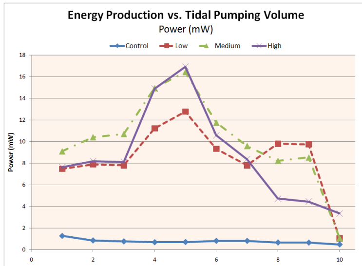
Figure 7. Tidal pumping through BMFCs
