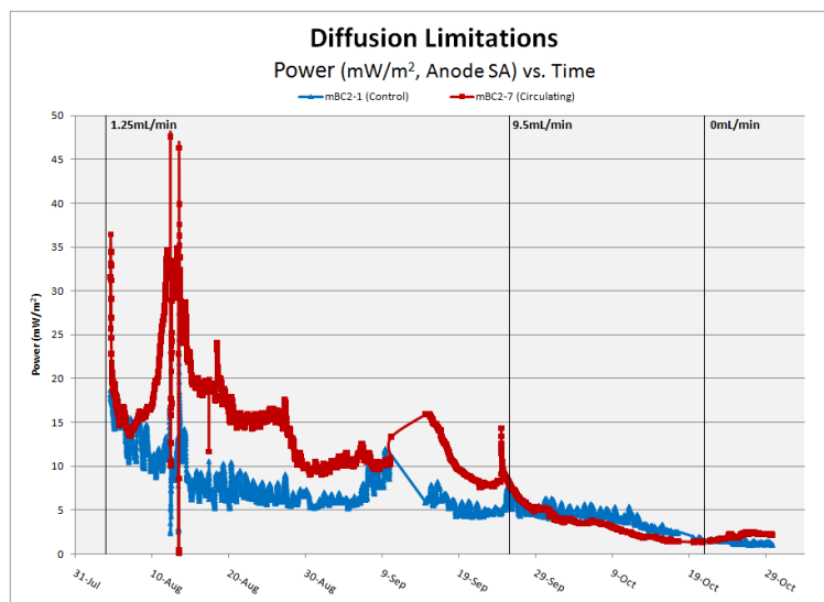
Figure 5. Mixing BMFC headspace to eliminate diffusion limitations
