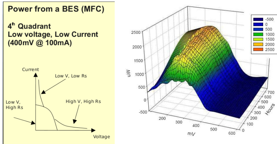
Figure 9. Graphical representation of MFC power quality
