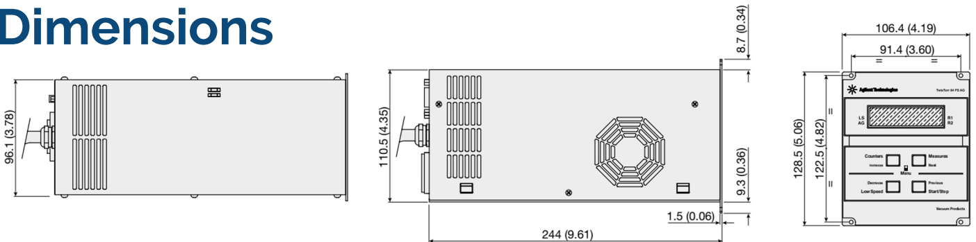
Dimensions: millimeters (inches)
