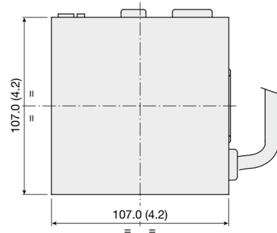
24 V controller front panel
