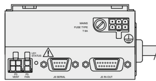
24 V controller front panel
