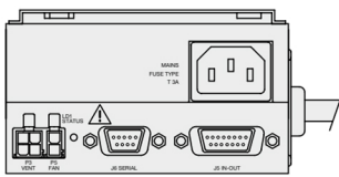
120/220 V controller front panel
