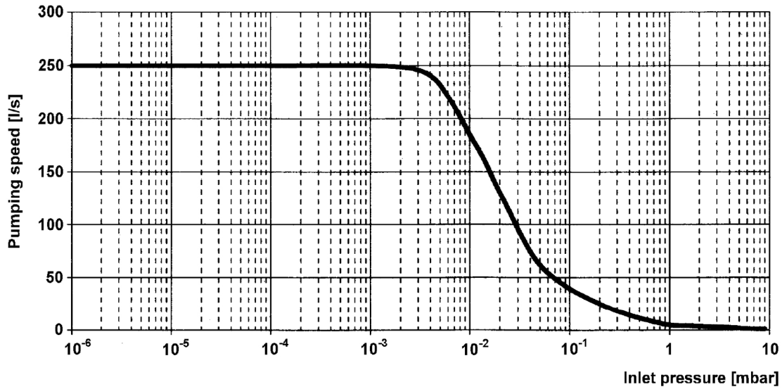
Graph of nitrogen pumping speed against inlet pressure
