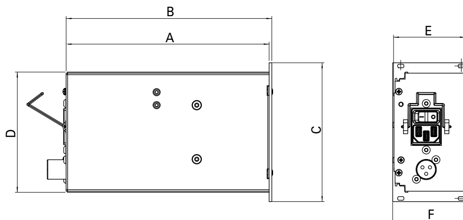
Fig. 4: Mains pack as 19" partial plug-in 3HU with front plate
