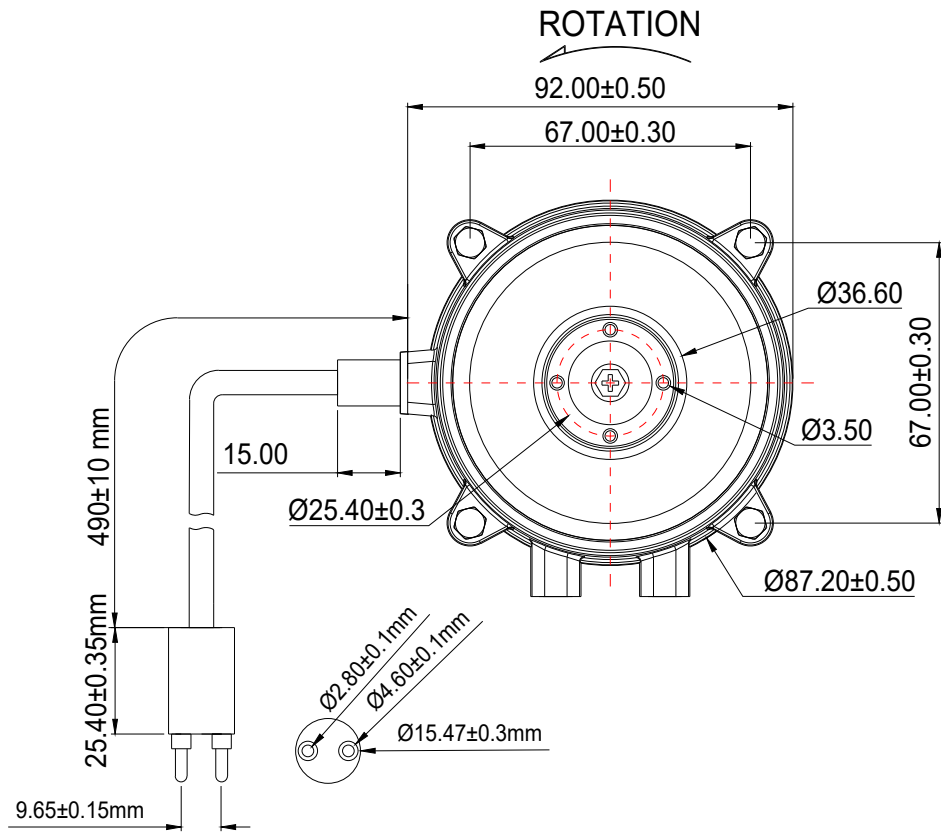
Cable Part Number BTHK105-0166 (Rev B)
