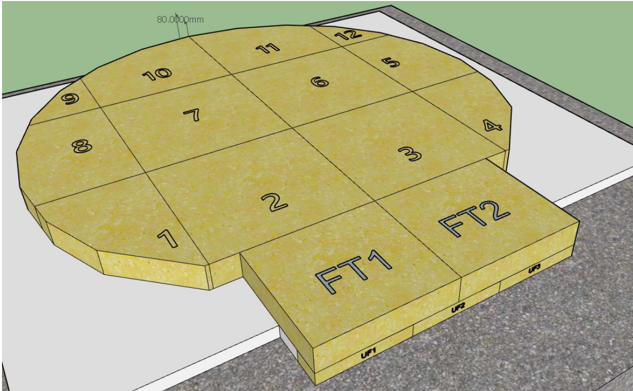
800 Floor tile layout
