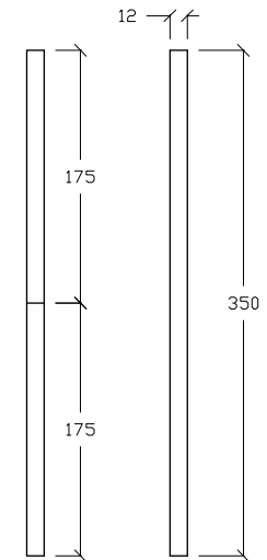
SIDE SECTION
