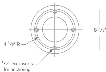
Anchor Bolt Plate
