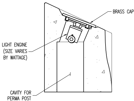
SECTION VIEW
