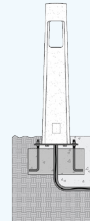
BG Lit and Non-Lit Bollards.
