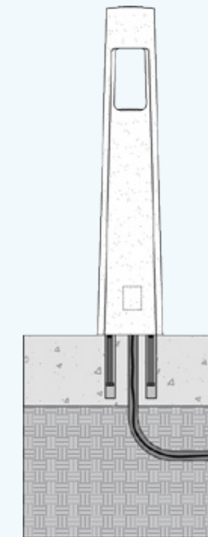
SM Lit and Non-Lit Bollards.
