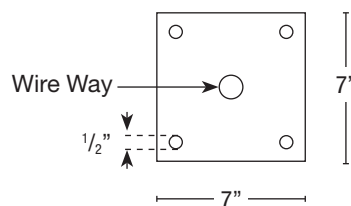
Anchor Bolt Pattern
