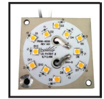
FB-MP1000 120V 10W 1000 LUMENS WARM DIMMING
