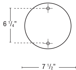
Anchor Bolt Pattern
