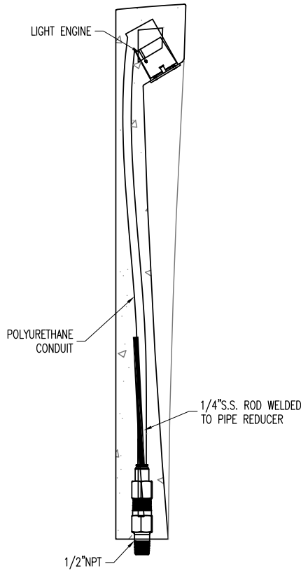
SECTION VIEW
