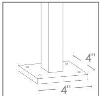
Model: DM4-1 Deck Mount or 1/2" NPT Option
