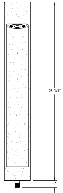
ELEVATION VIEW
