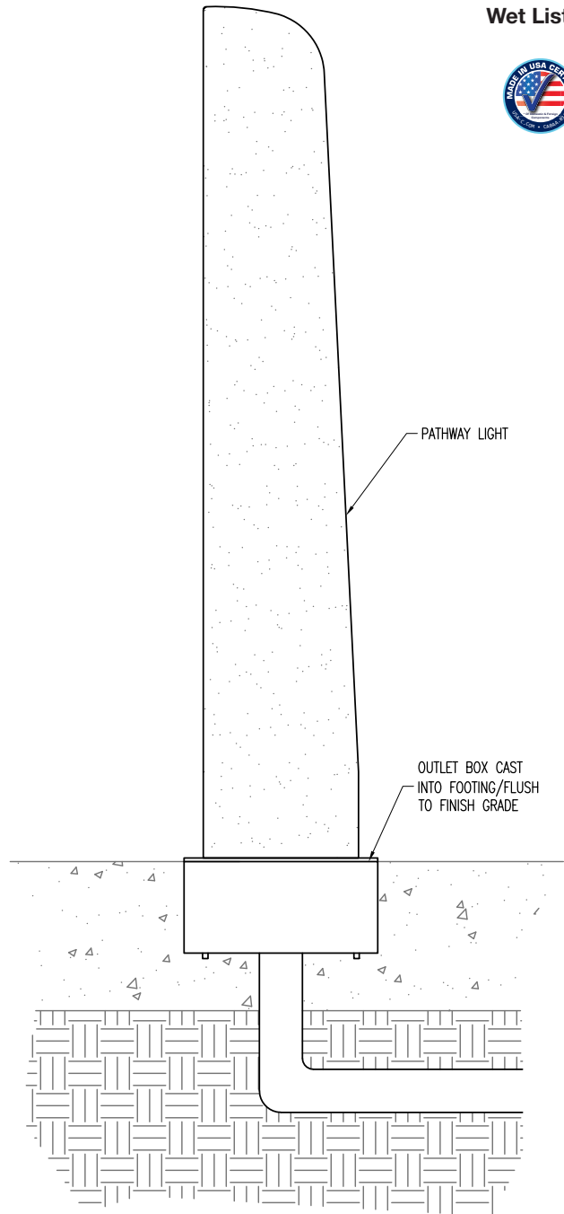
INSTALLATION SIDE VIEW N.T.S.
