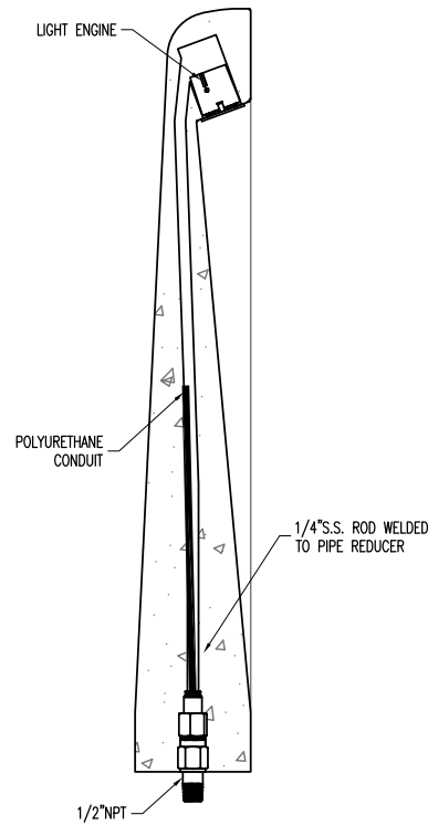
SECTION VIEW
