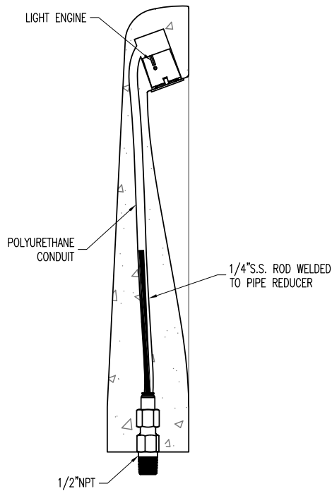
SECTION VIEW
