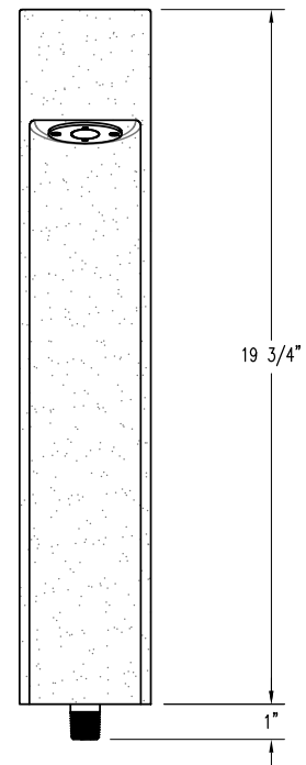
ELEVATION VIEW
