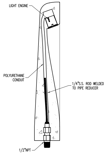
SECTION VIEW
