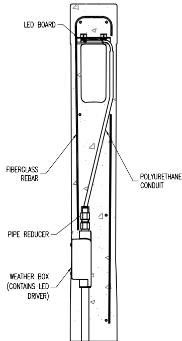
SECTION VIEW
