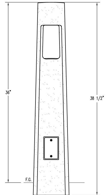
ELEVATION VIEW
