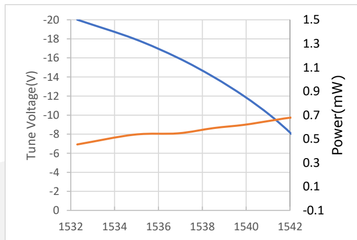
Wavelength Tuning Curve
