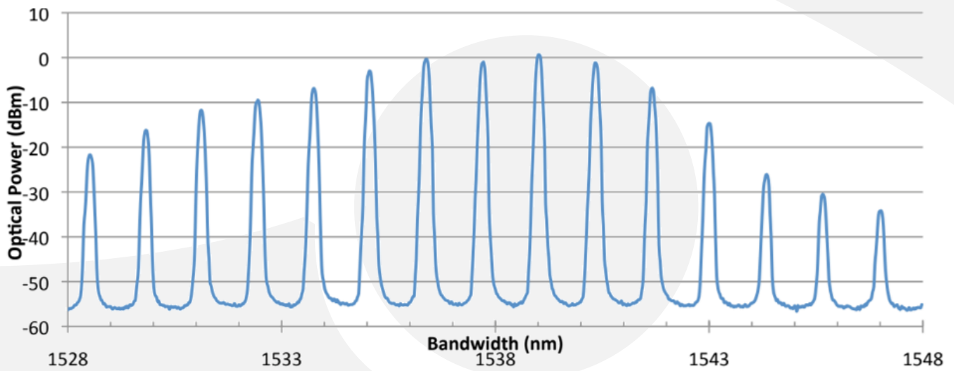
TYPICAL OPTICAL SPECTRUM @ 25°C @ 10 mW
