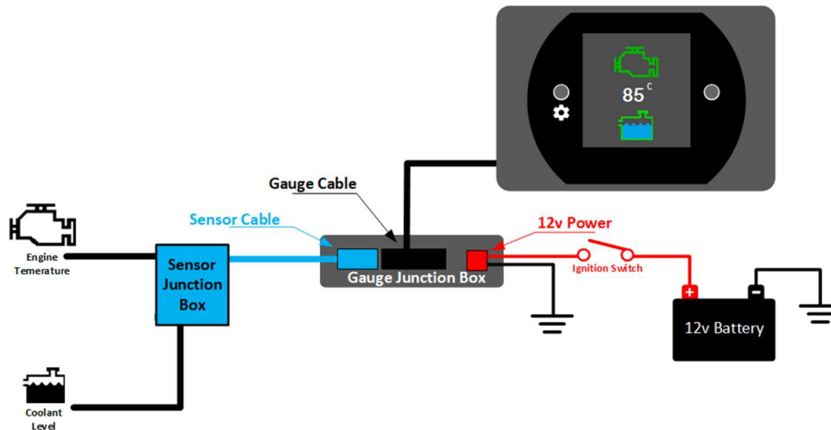
Wiring Diagram (gauge rear view)
