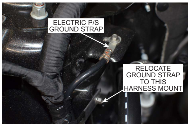
Fig. 7-e: Ground Strap Relocation
