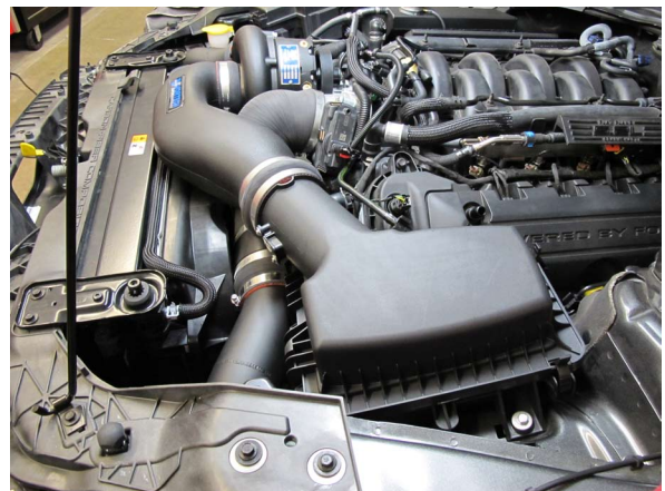
Fig. 8-f: Connect Inlet Duct To Air Box
