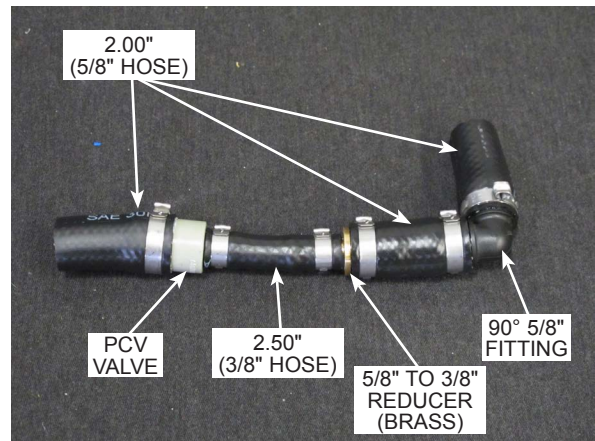
Fig. 4-b: PCV Assembly Layout
