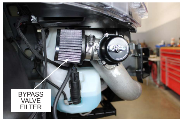
Fig. 5-i: Bypass Valve Mounting
