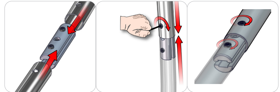
Connection Method 2: ES50
