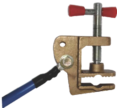
Alternative Screw Clamp detail
