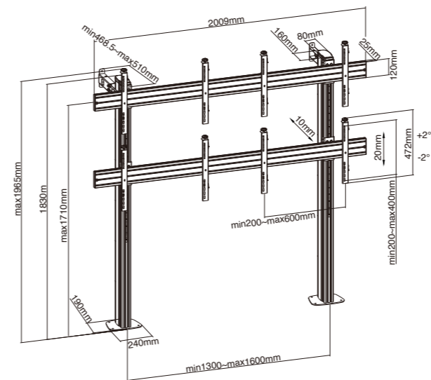
LVS02-446FB 2x2 / with Bolt-Down Base
