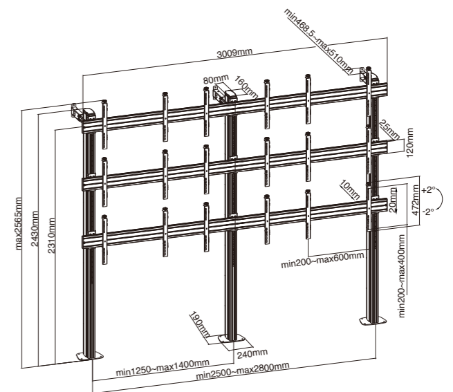
LVS02-946FB 3x3 / with Bolt-Down Base
