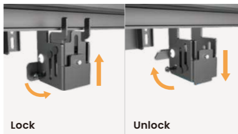
Quick-Release Latch easily activates lock & unlock mode to secure displays
