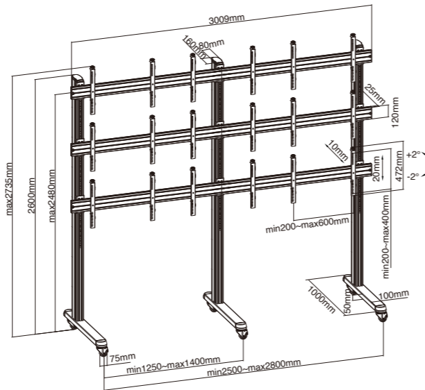
LVS02-946FW 3x3 / with Locking Casters
