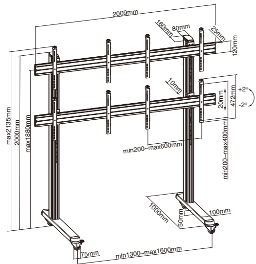
LVS02-446FW 2x2 / with Locking Casters
