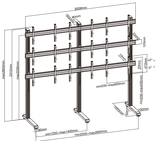
LVS02-946FF 3x3 / with Leveling Feet
