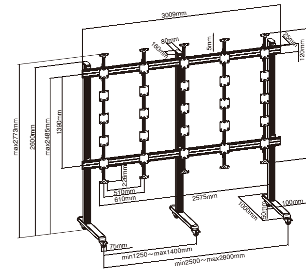
LES01-66AA 6x6 / For Absen Acclaim Series
