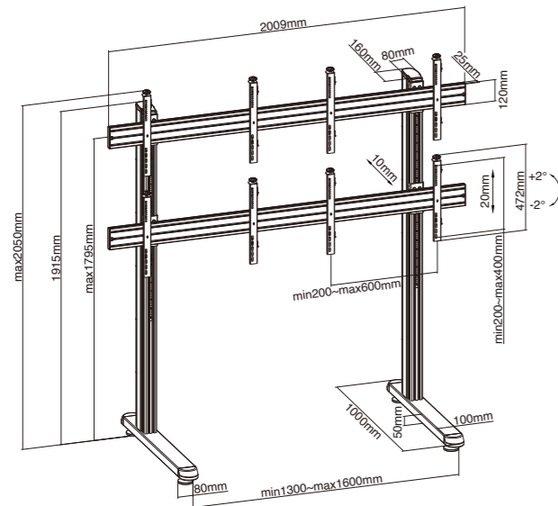
LVS02-446FF 2x2 / with Leveling Feet
