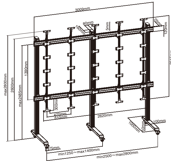
LES01-66UU 6x6 / For Unilumin Upanels Series
