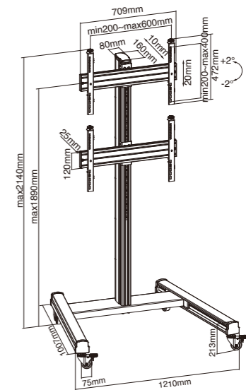
LVS02-246FW 1x2 / with Locking Casters
