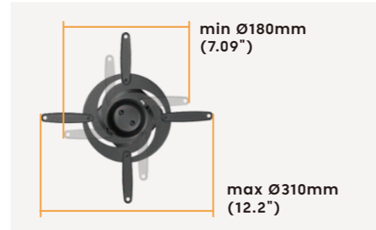
Adapter Arm Extension Range supports various projector sizes
